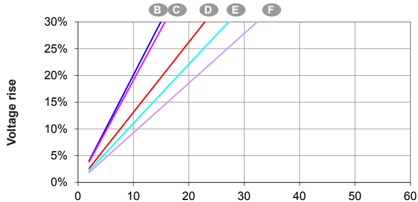
Load shedding (SHUNT and AREP) - kVA at P.F. = 0.8
